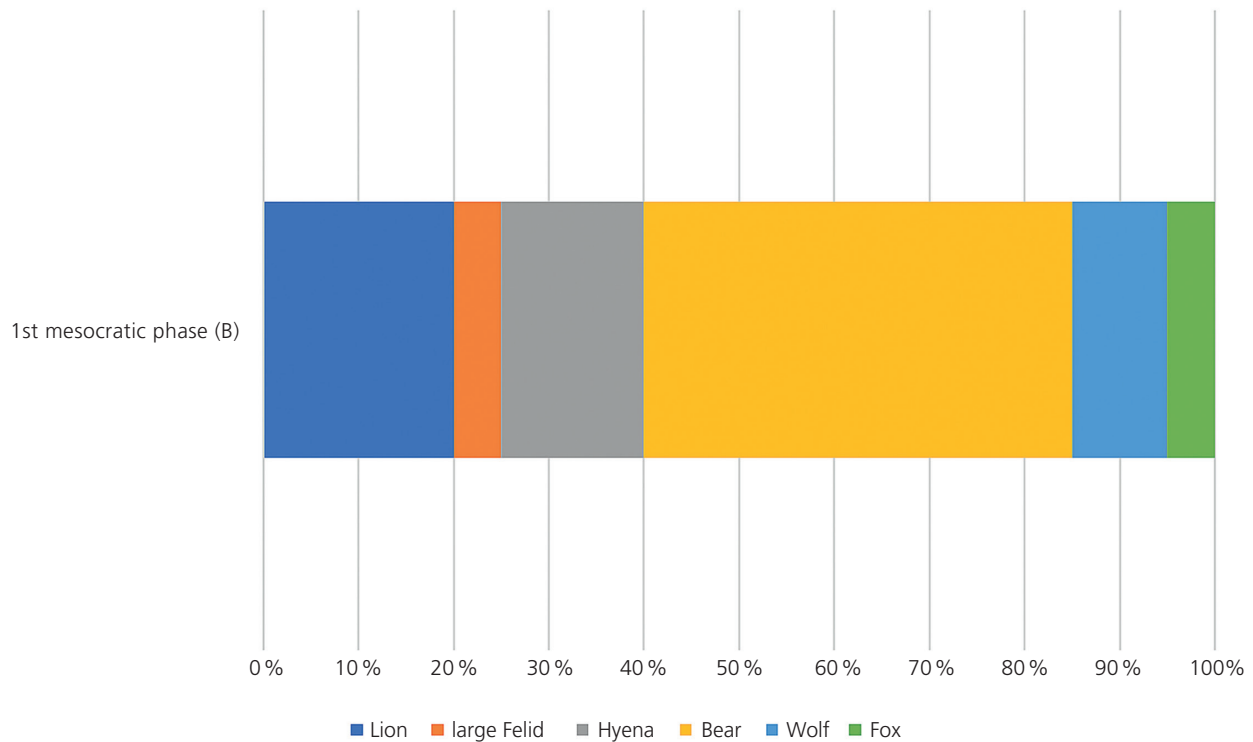
Fig. 7 Composition of the carnivore thanatocoenosis (based on estimates of MNI = minimum number of individuals) in the Neumark lakeland during the first mesocratic phase of the Eemian Interglacial Cycle.
