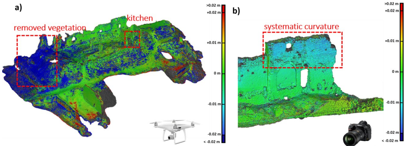
Fig. 7. Comparison of the laser scan point cloud with the a) drone-model and b) SLR model (© Bauer).
