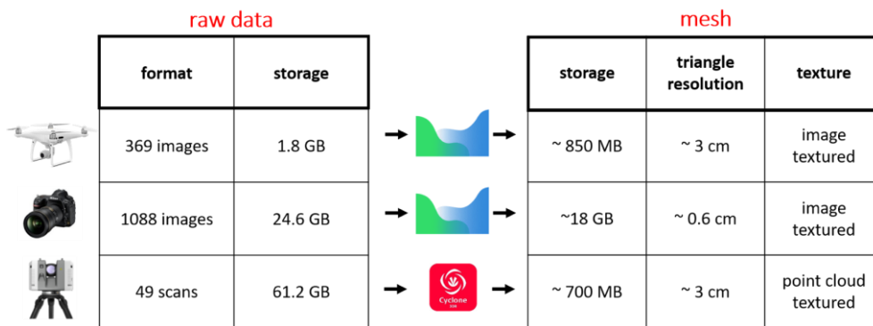
Fig. 5. Nominal differences in the meshing results of the technologies (© Bauer).
