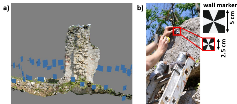
Fig. 3. a) camera positions for the documentatin of a late gothic pillar fragment b) mounting of the wall markers (© Kaufmann).
