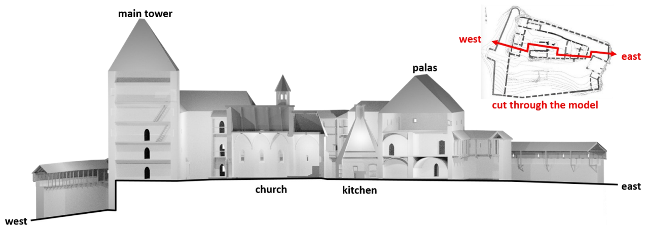
Fig. 10. Virtual reconstruction attempt of the castle Neu-Wildon (© Bauer).
