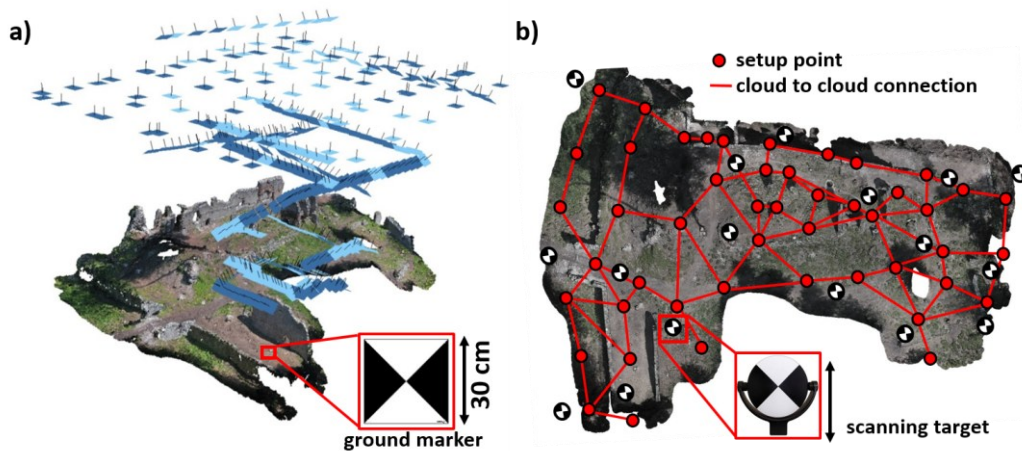
Fig. 4. a) Automatic flight mission with the DJI Phantom 4 (© Kaufmann) and b) setups of the laser scanning session (© Bauer).
