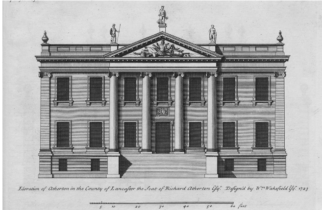
Abb. 36 Colen Campbell, Elevation of Atherton in the County of Lancaster
