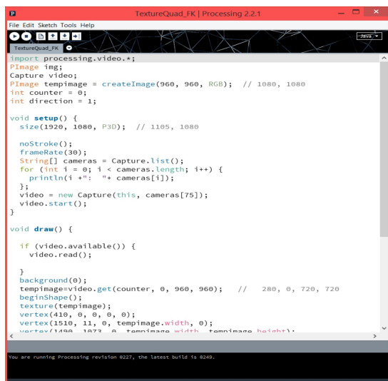
Fig. 5: Processing Texture Quad Sketch
